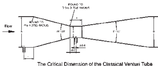
The Critical Dimension of the Classical Venturi Tube
